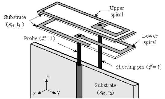
(a) 입체도 (a) 3-dimensional view
